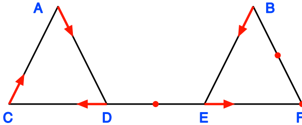
Fig. 1 Sample discrete vector field. This figure shows a simplicial complex \mathcal{X} which is a graph on six vertices with seven edges. Critical cells are indicated by red dots; vectors of the vector field are shown as red arrows (Color figure online)
